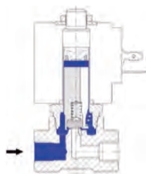
Bobina desenergizada / Coil de-energized Electroválvula cerrada / Solenoid valve closed
