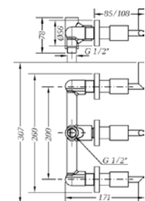
Ref.: 68116 12 45 66 Grupo ducha empotrado 8" con inversor Built-in 8" shower mixer with diverter
