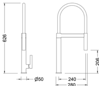
Ref.: 65219 40 60 66 Monomando de fregadera inox cartucho 25 Stainless steel single lever sink mixer 25 cartridge
