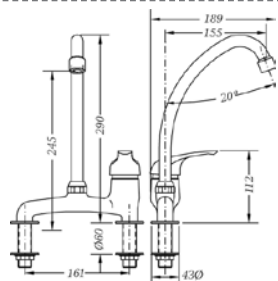
Ref.: 60199 05 45 66 Monomando mesada 16cm 16cm widespread single lever sink mixer Box: 1 | Carton: 10 | Pallet: 240
