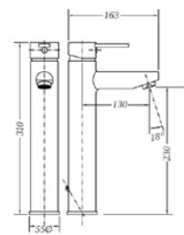
Ref.: 65136 29 45 66 Monomando de lavabo alto High single lever wash-basin mixer
