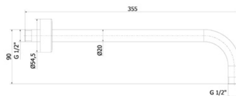
Ref.: B64113 43 Brazo pared redondo 35cm Bronce Bronze round wall arm 35cm
