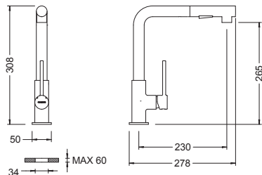
Ref.: FRV61208 45 Monomando de fregadera caño extraíble Tau Tau Single-lever sink mixer with pull-out spout
