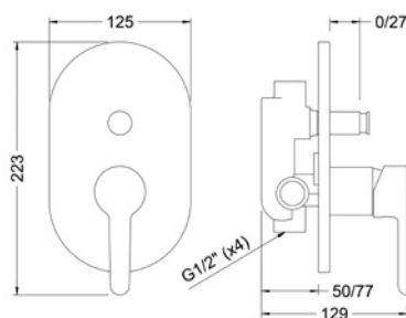
Ref.: 65116 19 45 66 Monomando empotrado con inversor 2 vías 2 way Built-in single lever mixer with diverter
