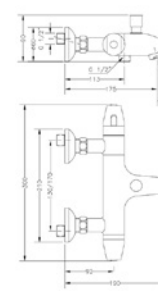
Ref.: 67103 14 45 67 Termostática baño Thermostatic bath mixer
