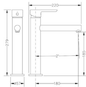
Ref.: 65134 19 41 66 Monomando de lavabo medio alto Medium height single lever wash-basin mixer
