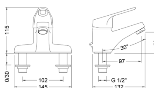
Ref.: 60188 22 45 66 Monomando de lavabo centerset 4" Single lever wash-basin mixer 4" centerset
