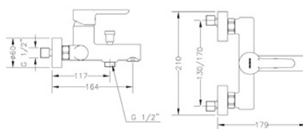
Ref.: 65100 19 45 66 Monomando de baño con kit Single lever bath mixer with kit
