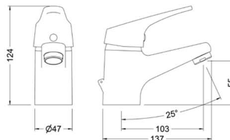
Ref.: 60130 22 45 66 Monomando de lavabo Single lever wash-basin mixer
