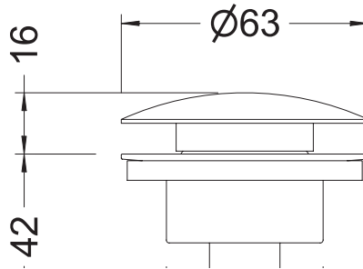
Ref.: 100202 45 Tapa universal "Click remove" "Click remove" universal cover
