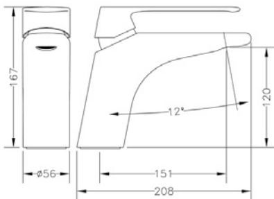
Ref.: 62130 08 45 66 Monomando de lavabo Single lever wash-basin mixer
