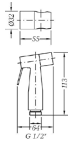
Ref.: 100694 41 Kit ducha sanitaria Negro Black Sanitary shower kit
