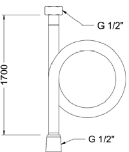
Ref.: 9908 0287 Flexo H 1/2" - H 1/2" 1,70 m inoxidable negro F 1/2" - F 1/2" Black stainless steel flexible hose 1.70 m
