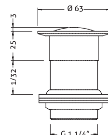
Ref.: 100207 45 Válvula universal lavabo y bidé click Click pop-up waste for basin and bidet
