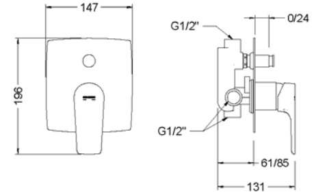
Ref.: 64116 32 45 66 Monomando empotrado con inversor 2 vías 2 way Built-in single lever mixer with diverter
