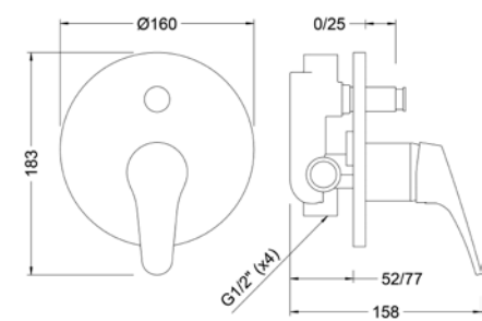
Ref.: 61116 22 45 66 Monomando empotrado con inversor 2 vías 2 way Built-in single lever mixer with diverter Box: 1 | Carton: 12 | Pallet: 216
