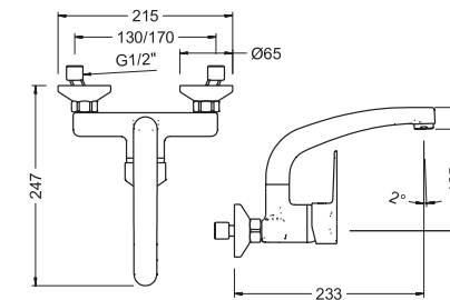
Ref.: 61190 28 45 66 Monomando de fregadera mural 15 cm caño corto Wall single lever sink mixer 15 cm short spout
