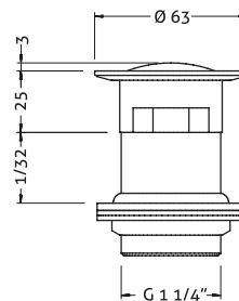
Ref.: 100206 45 Válvula universal click lavabo y bidé click con rebosadero Click pop-up waste for basin and bidet with overflow
