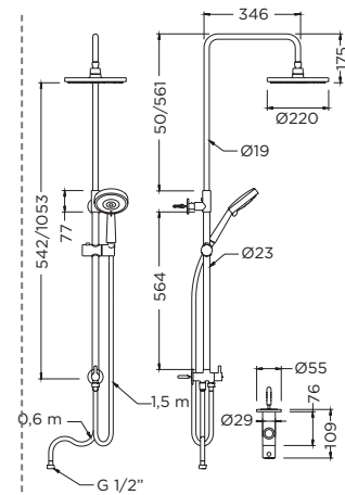
Ref.: 1745 45 Set columna con ducha, soporte y flexo Column set with shower, holder and flexible hose Box: 1 | Carton: 2 | Pallet: 8
