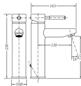
Ref.: 65134 18 45 66 Monomando de lavabo medio alto Medium height single lever wash-basin mixer
