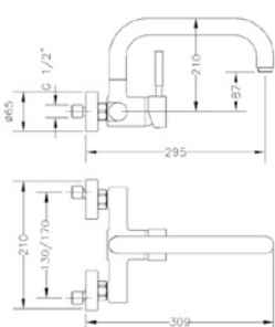
Ref.: 65192 18 45 66 Monomando de fregadera mural 15 cm Wall single lever sink mixer 15 cm Box: 1 | Carton: 4 | Pallet: 72
