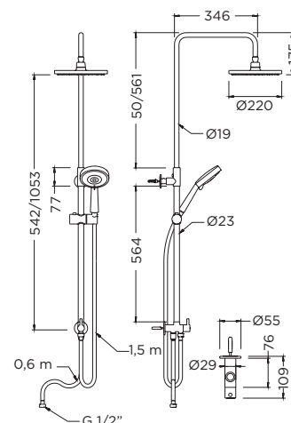
Ref.: 1745 45 Set columna con ducha, soporte y flexo Column set with shower, holder and flexible hose
