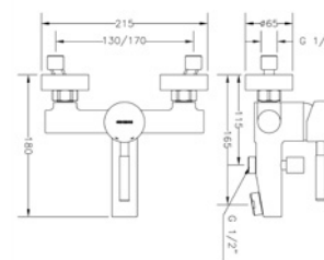
Ref.: 65100 18 45 66 Monomando de baño con kit Single lever bath mixer with kit
