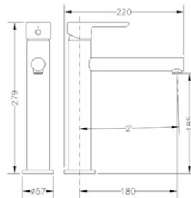
Ref.: 65134 19 45 66 Monomando de lavabo medio alto Medium height single lever wash-basin mixer
