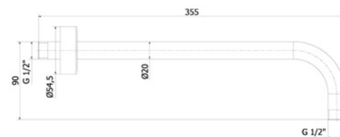
Ref.: B64113 43 Brazo pared redondo 35cm Bronze Bronze round wall arm 35cm Box: 1 | Carton: 1
