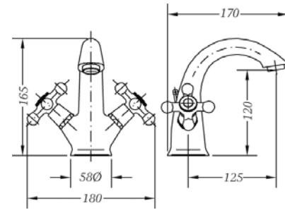
Ref.: 68506 09 43 66 Monobloc de lavabo bronce Bronze wash-basin mixer
