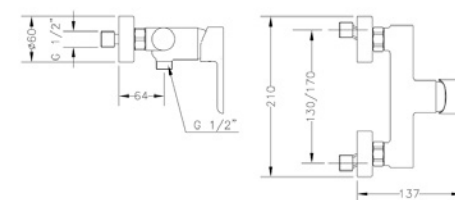
Ref.: 65110 19 45 66 Monomando de ducha con kit Single lever shower mixer with kit
