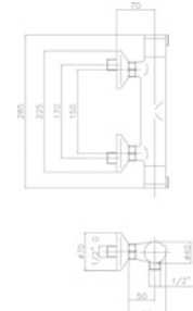
Ref.: 67112 14 45 67 Termostática ducha Thermostatic shower mixer
