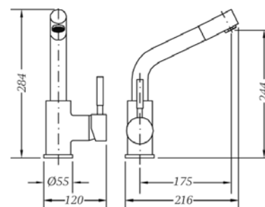
Ref.: 65206 18 45 66 Monomando de fregadera caño extraíble Single lever sink mixer with pull-out spout Box: 1 | Carton: 8 | Pallet: 192
