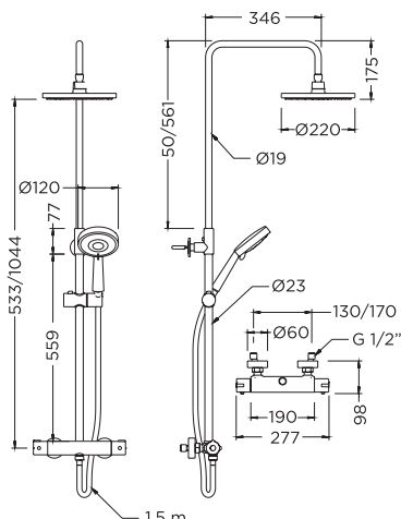
Ref.: CT67110 18 Columna termostática extensible con kit Thermostatic extendable column with kit
