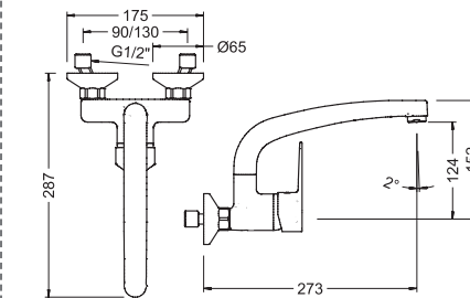
Ref.: 61195 28 45 66 Monomando de fregadera mural 11 cm Wall single lever sink mixer 11 cm
