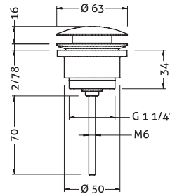
Ref.: 100211 43 Válvula universal click Luxe con y sin rebosadero bronce Bronze Luxe universal click pop-up waste with and without overflow
