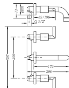
Ref.: 68131 12 45 66 Grupo de lavabo empotrado caño 16 cm Built-in wash-basin mixer with 16 cm pipe spout
