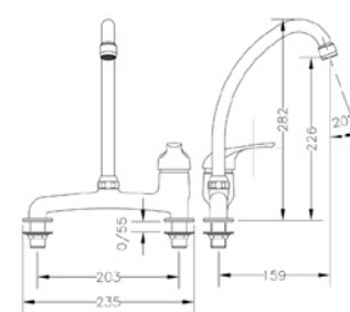
Ref.: 60198 05 45 66 Monomando mesada 8" 8" widespread single lever sink mixer Box: 1 | Carton: 6 | Pallet: 144
