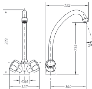
Ref.: 68200 11 45 66 Monobloc fregadera caño tubo Sink mixer, swan neck spout
