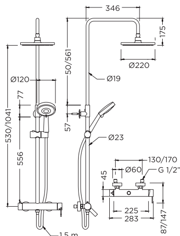
Ref.: CM65110 29 Columna monomando extensible con kit Single lever extendable column with kit
