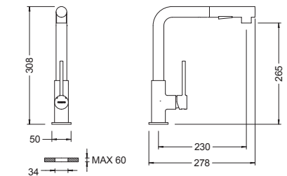
Ref.: FRV61208 44 Monomando de fregadera caño extraíble acabado Acero Inoxidable Tau Tau Stainless steel finish single-lever sink mixer with pull-out spout
