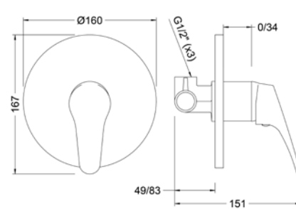
Ref.: 61115 22 45 66 Monomando de ducha empotrado Built-in single lever shower mixer Box: 1 | Carton: 12 | Pallet: 216
