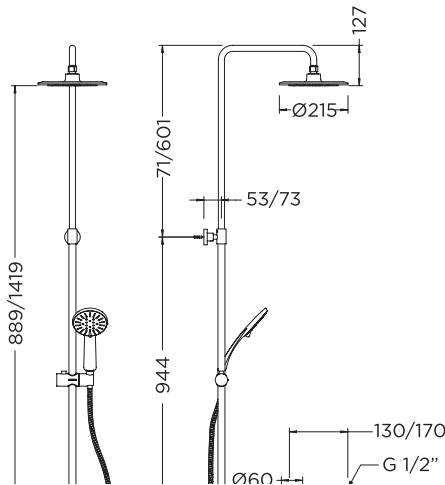
Ref.: CM65111 19 41 Columna monomando extensible con kit Single lever extensible column with kit
