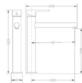
Ref.: 65136 19 45 66 Monomando de lavabo alto High single lever wash-basin mixer
