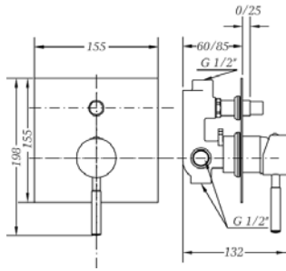
Ref.: 65116 18 45 66 Monomando empotrado con inversor 2 vías 2 way Built-in single lever mixer with diverter Box: 1 | Carton: 12 | Pallet: 216
