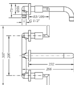
Ref.: 68132 12 45 66 Grupo de lavabo empotrado caño 22 cm Built-in wash-basin mixer with 22 cm pipe spout
