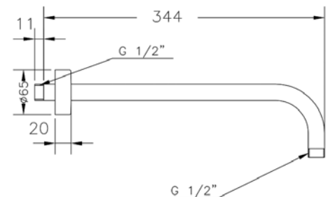
Ref.: B65113 18 Brazo pared redondo 35 cm Round wall arm 35 cm
