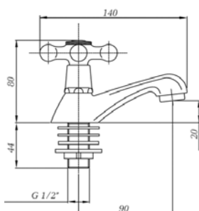
Ref.: 68500 09 45 66 Grifo lavabo Wash-basin tap
