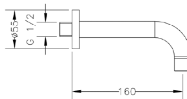
Ref.: 68911 45 Caño mural tubo recto 16 cm Wall-mounted pipe spout 16 cm Box: 1 | Carton: 40 | Pallet: 640
