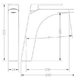
Ref.: 62136 08 45 66 Monomando de lavabo alto High single lever wash-basin mixer
