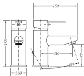
Ref.: 65135 29 45 66 Monomando de lavabo Single lever wash-basin mixer
