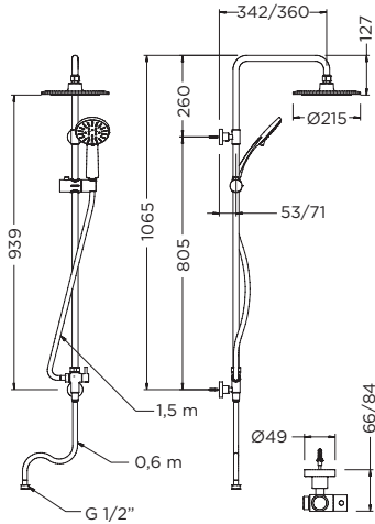
Ref.: 1744 41 Set columna fija con kit Fixed column set with kit
