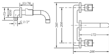
Ref.: 68131 07 45 66 Grupo de lavabo empotrado caño 16 cm Built-in wash-basin mixer with 16 cm pipe spout
