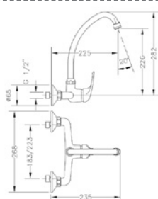
Ref.: 60194 05 45 66 Monomando de fregadera mural 8" Wall single lever 8" sink mixer Box: 1 | Carton: 6 | Pallet: 216
