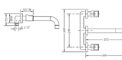
Ref.: 68132 07 45 66 Grupo de lavabo empotrado caño 22 cm Built-in wash-basin with 22 cm pipe spout
