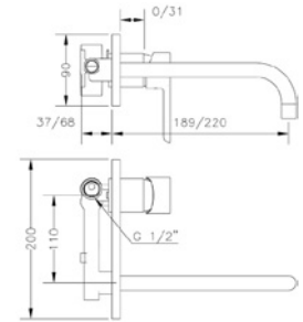
Ref.: 65132 19 41 66 Monomando de lavabo empotrado caño 22cm Built-in wash-basin mixer 22 cm spout
