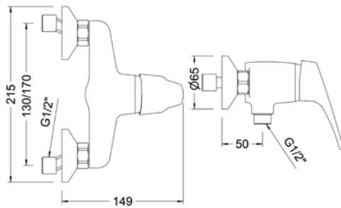
Ref.: 60110 22 45 66 Monomando de ducha con kit Single lever shower mixer with kit Box: 1 | Carton: 8 | Pallet: 160
