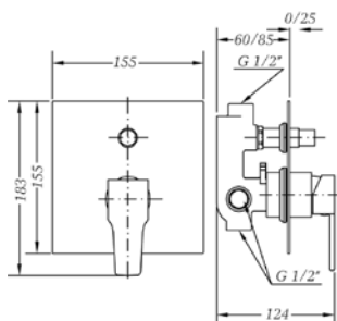
Ref.: 63116 26 45 66 Monomando empotrado con inversor 2 vías 2 way Built-in single lever mixer with diverter
