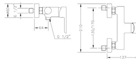
Ref.: 65110 19 41 66 Monomando de ducha con kit Single lever shower mixer with kit
