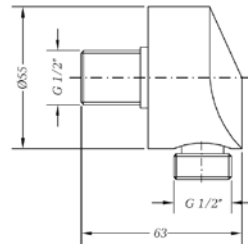
Ref.: 1680 04 Toma ducha mural redonda Round wall connector Box: 1 | Carton: 40 | Pallet: 2304
