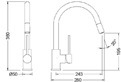
Ref.: FRV61207 41 Monomando de fregadera caño extraíble Tau Tau Single-lever sink mixer with pull-out spout
