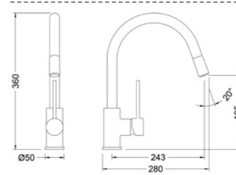
Ref.: FRV61206 Monomando de fregadera caño extraíble Single-lever sink mixer with pull-out spout Box: 1 | Carton: 4 | Pallet: 48
