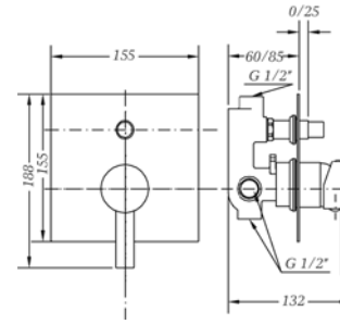
Ref.: 65116 29 45 66 Monomando empotrado con inversor 2 vías 2 way Built-in single lever mixer with diverter
