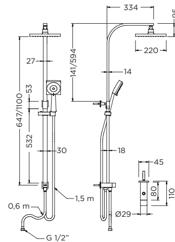
Ref.: 1746 45 Set columna con ducha, soporte y flexo Column set with shower, holder and flexible hose
