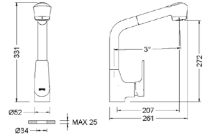
Ref.: 64206 32 45 66 Monomando de fregadera ducha extraíble Korál Korál Single lever sink mixer with pull-out spray
