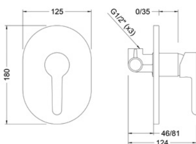
Ref.: 65115 19 41 66 Monomando empotrado con inversor 2 vías 2 way Built-in single lever mixer with diverter
