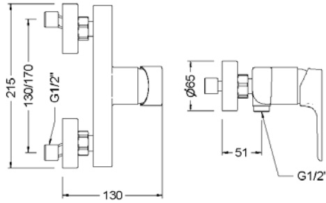
Ref.: 64110 32 45 66 Monomando de ducha con kit Single lever shower mixer with kit
