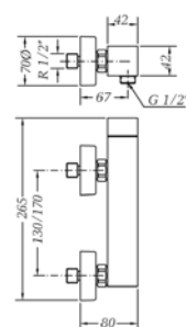
Ref.: 63110 26 45 67 Monomando de ducha sin kit Single lever shower mixer without kit
