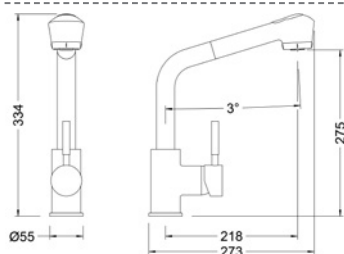
Ref.: 65205 18 45 66 Monomando de fregadera ducha extraíble Single lever sink mixer with pull-out spray Box: 1 | Carton: 6 | Pallet: 108
