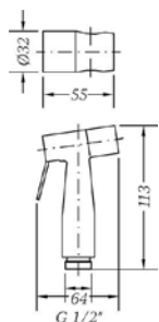
Ref.: 100694 41 Kit ducha sanitaria Negro Black Sanitary shower kit
