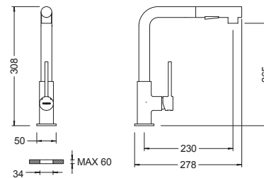
Ref.: FRV61208 41 Monomando de fregadera caño extraíble Tau Negra Tau Black single-lever sink mixer with pull-out spout
