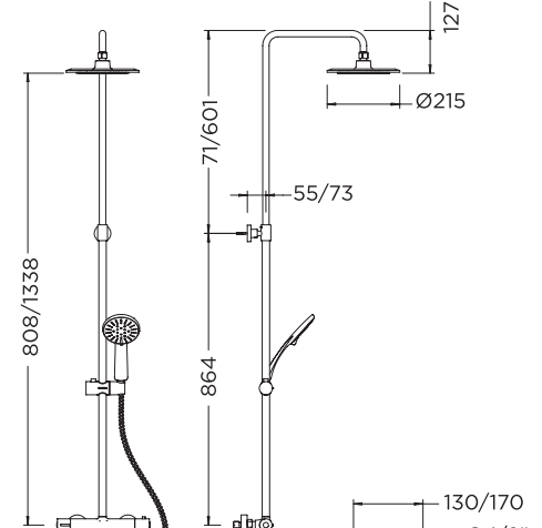
Ref.: CT67111 19 41 Columna termostática extensible con kit Thermostatic extensible column with kit
