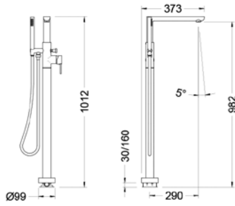
Ref.: 65119 29 45 66 Monomando de pie para bañera Tau 2 Tau 2 Floor single lever mixer for bath
