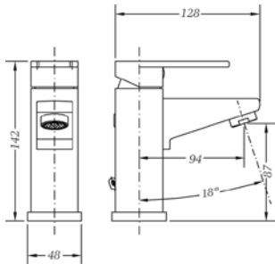
Ref.: 63130 26 45 66 Monomando de lavabo Single lever wash-basin mixer Box: 1 | Carton: 20 | Pallet: 360
