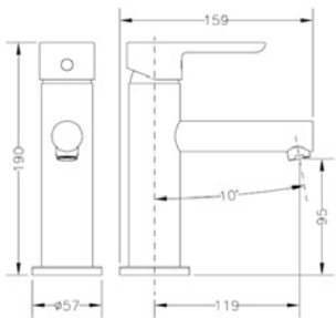
Ref.: 65130 19 45 66 Monomando de lavabo Single lever wash-basin mixer
