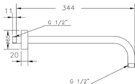
Ref.: B65113 18 Brazo pared redondo 35 cm Round wall arm 35 cm Box: 1 | Carton: 20 | Pallet: 600
