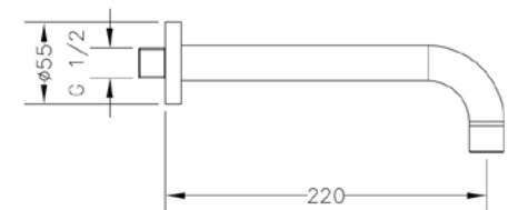
Ref.: 68912 45 Caño mural tubo recto 22 cm Wall-mounted pipe spout 22 cm Box: 1 | Carton: 40 | Pallet: 640
