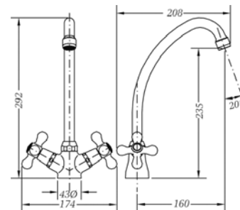
Ref.: 68540 09 45 66 Monobloc fregadera caño tubo Sink mixer, swan neck spout
