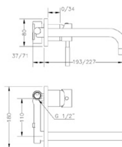
Ref.: 65132 18 45 66 Monomando de lavabo empotrado caño 22 cm Built-in wash-basin mixer 22 cm spout
