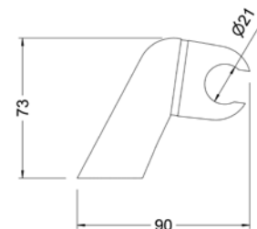
Ref.: 100152 45 00 Soporte ducha Shower holder
