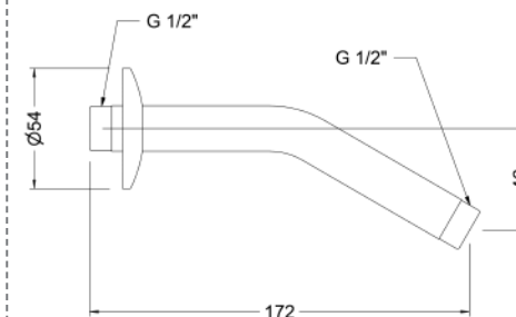
Ref.: 1699 45 00 Brazo pared redondo 12 cm Round wall arm 12 cm Box: 5 | Carton: 75 | Pallet: 2700
