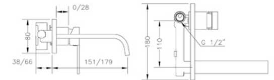
Ref.: 63131 26 45 66 Monomando de lavabo empotrado caño 16 cm Built-in wash-basin mixer 16 cm spout
