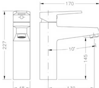
Ref.: 64134 16 45 66 Monomando de lavabo medio alto Medium height single lever wash-basin mixer
