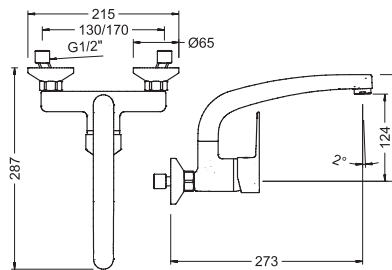
Ref.: 61192 28 45 66 Monomando de fregadera mural 15 cm Wall single-lever sink mixer 15 cm
