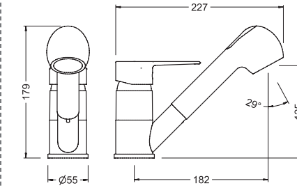
Ref.: 61205 28 45 66 Monomando de fregadera ducha extraíble Single lever sink mixer with pull-out spray
