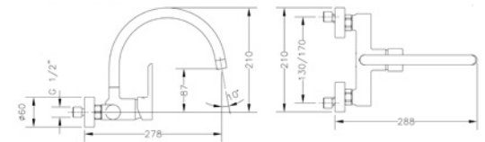
Ref.: 65192 19 45 66 Monomando de fregadera mural 15 cm Wall single lever sink mixer 15 cm
