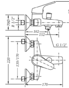
Ref.: 60100 22 45 66 Monomando de baño con kit Single lever bath mixer with kit Box: 1 | Carton: 8 | Pallet: 128
