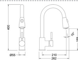
Ref.: FRV61205 Monomando de fregadera ducha extraíble Single lever sink mixer with pull-out spray Box: 1 | Carton: 4 | Pallet: 72
