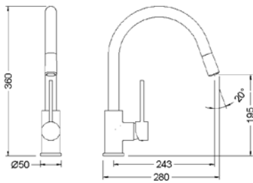
Ref.: FRV61206 Monomando de fregadera caño extraíble Tau Tau Single-lever sink mixer with pull-out spout
