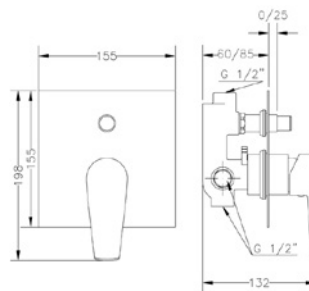
Ref.: 64116 16 45 66 Monomando empotrado con inversor 2 vías 2 way Built-in single lever mixer with diverter
