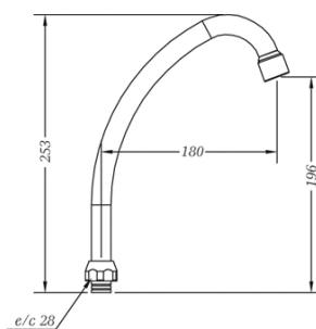
Ref.: 68903 45 Caño tubo vertical Vertical pipe spout
