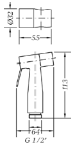
Ref.: 100694 60 Kit ducha sanitaria inox Stainless steel sanitary shower kit Box: 1 | Carton: 22 | Pallet: 264
