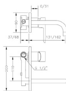
Ref.: 65131 19 45 66 Monomando de lavabo empotrado caño 16 cm Built-in wash-basin mixer 16 cm spout
