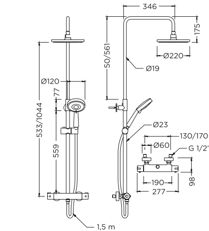
Ref.: CT67110 18 Columna termostática extensible con kit Thermostatic extensible column with kit Box: 1 | Carton: 2 | Pallet: 8
