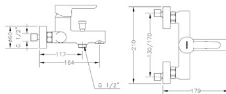
Ref.: 65100 19 41 66 Monomando de baño con kit Single lever bath mixer with kit
