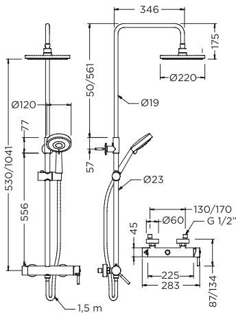
Ref.: CM65110 18 Columna monomando extensible con kit Single lever extensible column with kit Box: 1 | Carton: 2 | Pallet: 8
