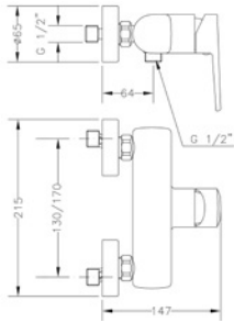
Ref.: 64110 04 45 66 Monomando de ducha con kit Single lever shower mixer with kit
