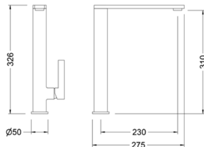
Ref.: 65215 40 60 66 Monomando de fregadera inox cartucho 25 Stainless steel single lever sink mixer 25 cartridge
