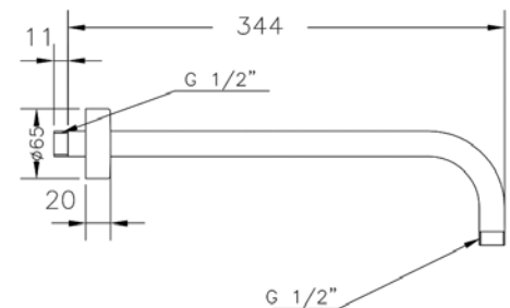
Ref.: B65114 18 Brazo pared redondo 24 cm Round wall 24 cm
