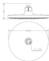
Ref.: R65112 18 Rociador redondo 22 cm Round shower head Ø 22 cm Box: 1 | Carton: 24 | Pallet: 144
