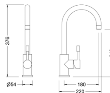
Ref.: 65203 18 60 66 Monomando de fregadera inox caño cisne Stainless steel single lever sink mixer with swan pipe
