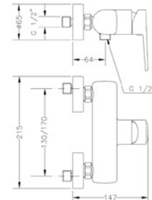
Ref.: 64110 16 45 66 Monomando de ducha con kit Single lever shower mixer with kit
