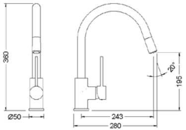
Ref.: FRV61207 44 Monomando de fregadera caño extraíble acabado Acero Inoxidable Tau Tau Stainless steel finish single-lever sink mixer with pull-out spout
