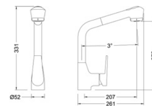
Ref.: 64206 16 45 66 Monomando de fregadera ducha extraíble Single lever sink mixer with pull-out spray
