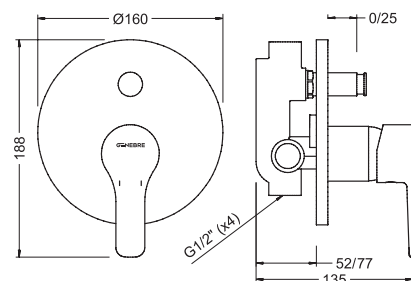
Ref.: 61116 28 45 66 Monomando empotrado con inversor 2 vías 2 way Built-in single lever mixer with diverter
