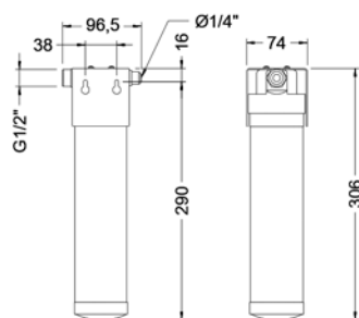
Ref.: FT00 Kit declorador Dechlorinator kit
