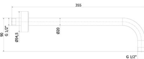
Ref.: B64113 41 Brazo pared redondo 35 cm negro Black round wall arm 35 cm Box: 1 | Carton: 20 | Pallet: 600
