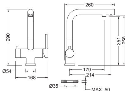
Ref.: 65703 18 60 66 Monomando de fregadera inox 3 vías Stainless steel single lever 3-way sink mixer Box: 1 | Carton: 4 | Pallet: 48
