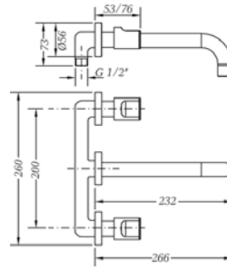
Ref.: 68132 08 45 66 Grupo de lavabo empotrado caño 22 cm Built-in wash-basin mixer with 22cm pipe spout
