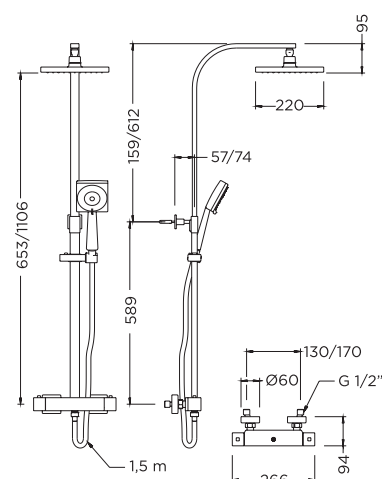
Ref.: CT67110 26 Columna termostática extensible con kit Thermostatic extendable column with kit
