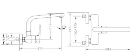
Ref.: 64192 16 45 66 Monomando de fregadera mural Wall single lever sink mixer
