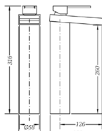
Ref.: 63138 26 45 66 Monomando de lavabo cascada alto High waterfall single lever wash-basin mixer
