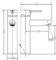
Ref.: 65134 29 45 66 Monomando de lavabo medio alto Medium height single lever wash-basin mixer
