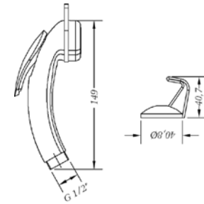
Ref.: 100696 45 Kit ducha sanitaria Sanitary shower kit Box: 1 | Carton: 100 | Pallet: 1800
